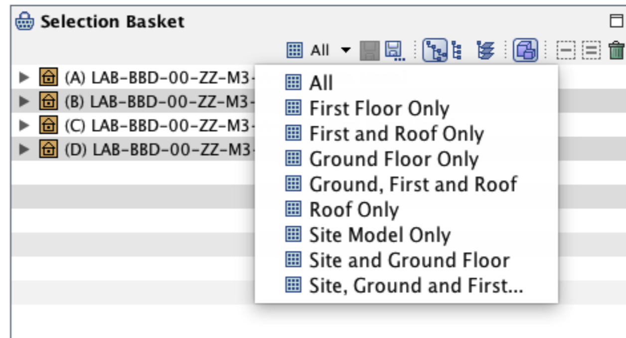
Model Filtering
