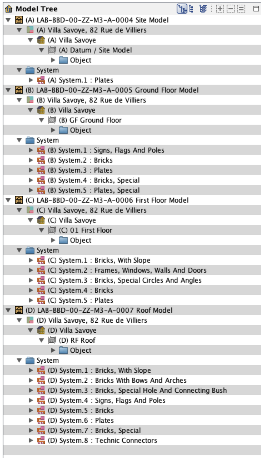
Model Tree
